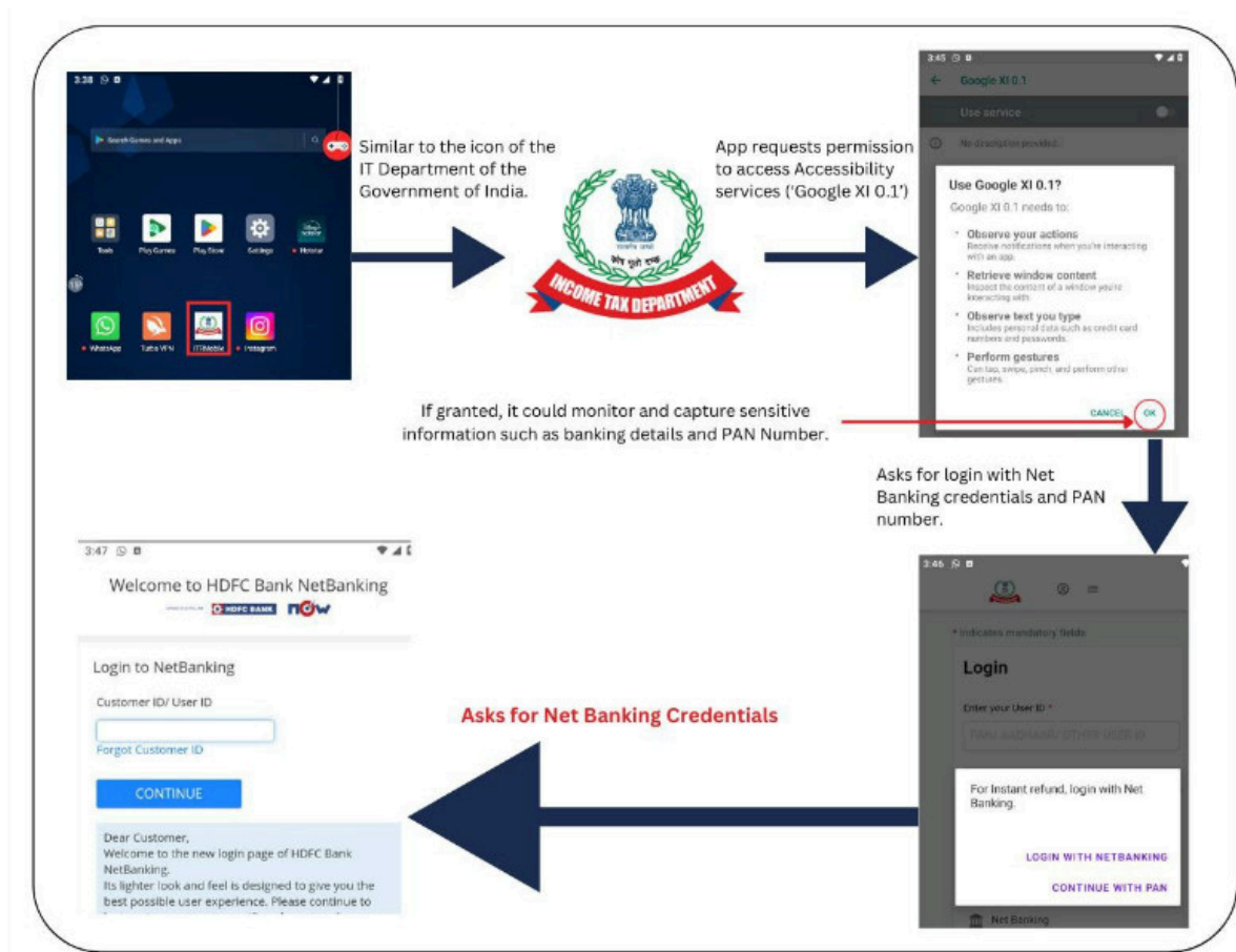
Fig. 2.1 A case of a malicious app
